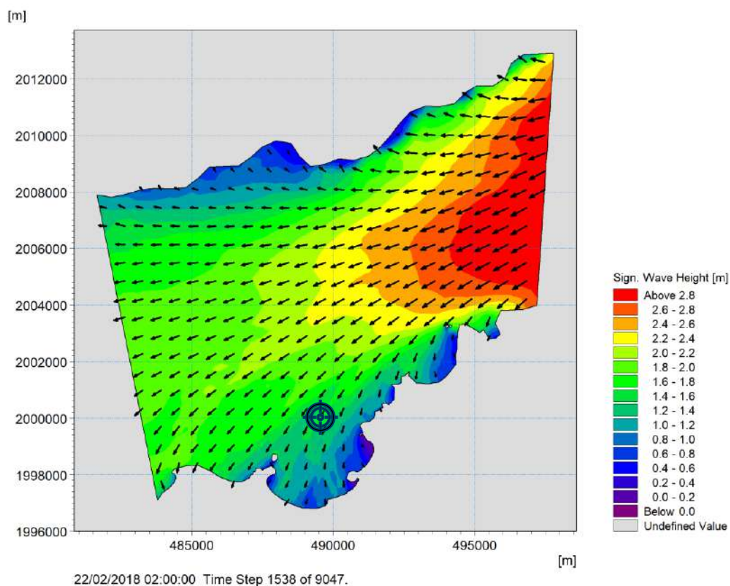
Figure 4.12 Champ de propagation des vagues le 22/02/2018 02h UTC (Alizé).
